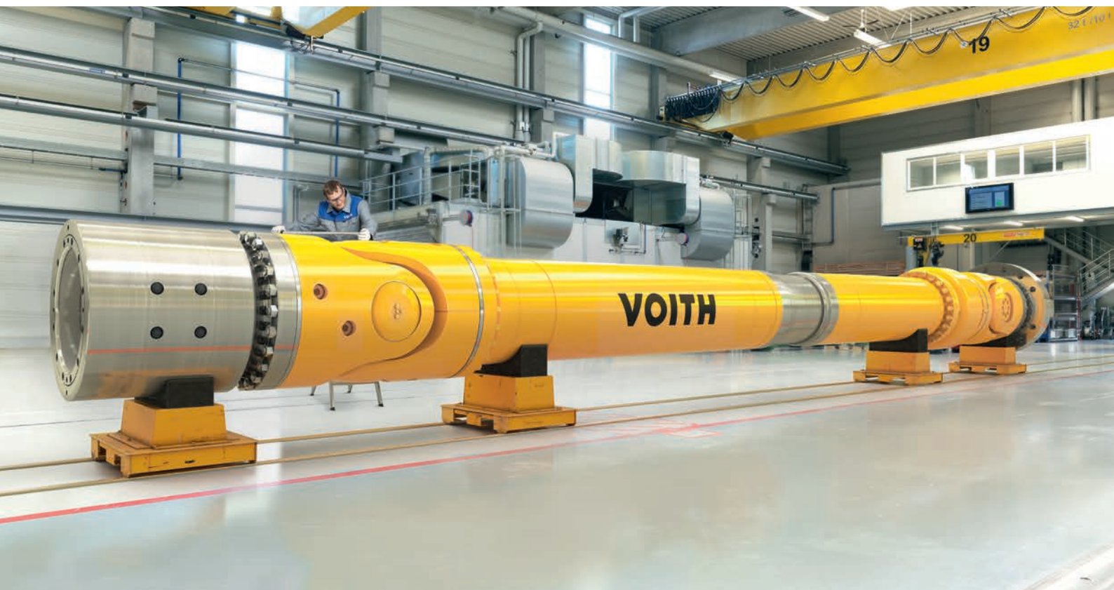
High-performance universal joint shafts in the assembly hall; E joint (left)
