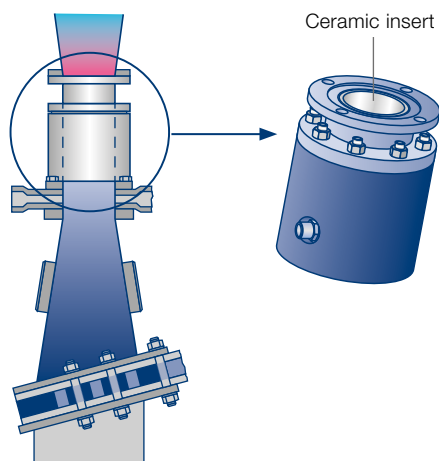
With vortex breaker
