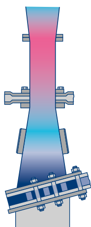
Without vortex breaker
