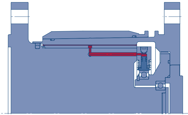
SA-P, flange to flange connection
