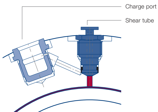
Pressure charge port (dual ports on SafeSet EZi)
