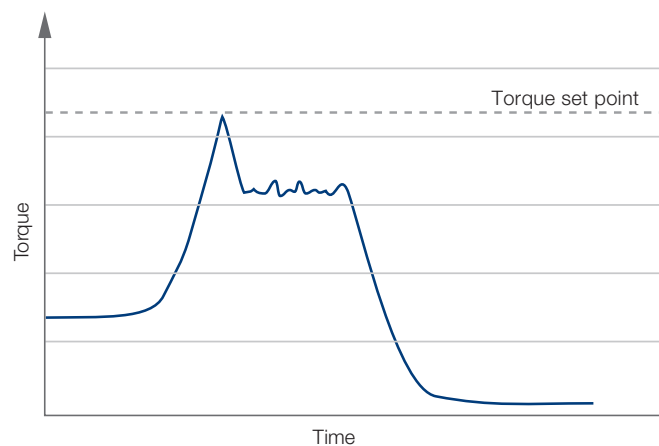
Typical release curve SafeSet
