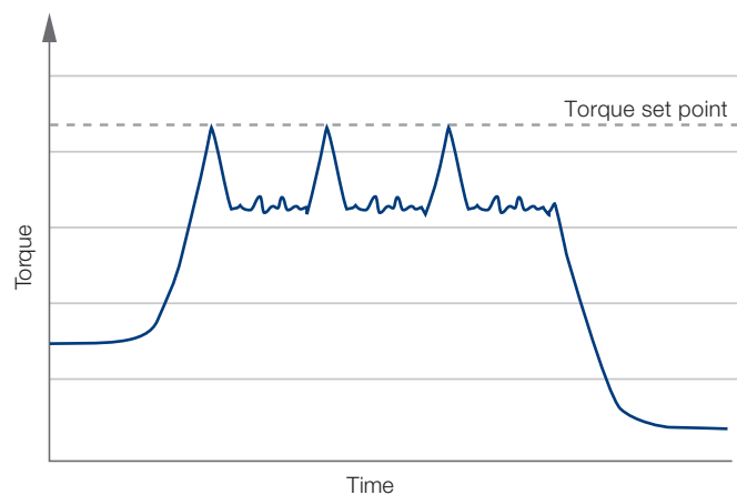
Typical release curve SafeSet EZi
