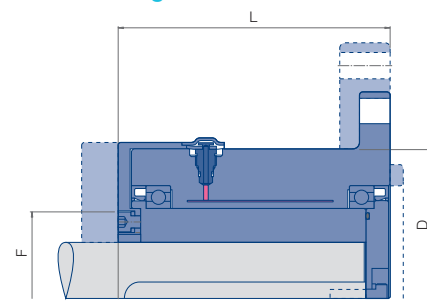
SafeSet EZi-K series, for keyway shaft to flange connections
