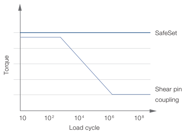
Fatigue curve (S-N curve)
